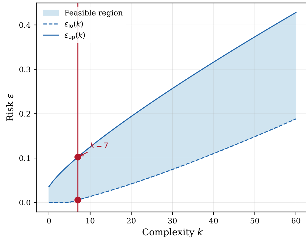
(b) Risk bounds ( N = 200 , \beta = 0.01 )
