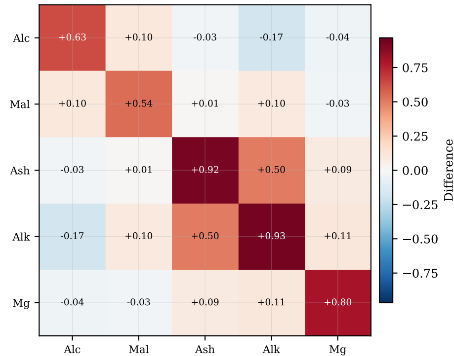
(a) \hat{\Sigma} - \Sigma_{\text{full}} (entry errors)
