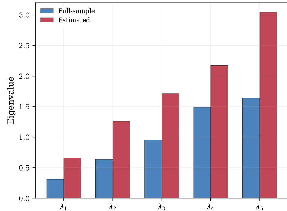
(c) Eigenvalue spectrum of \hat{\Sigma}
