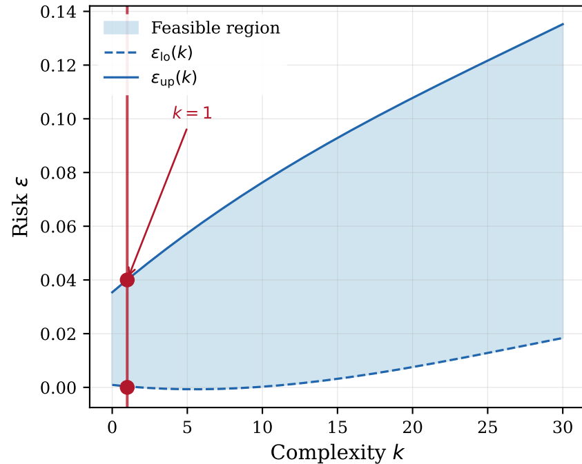
(b) Risk bounds ( N = 500, \beta = 10^{-6} )
