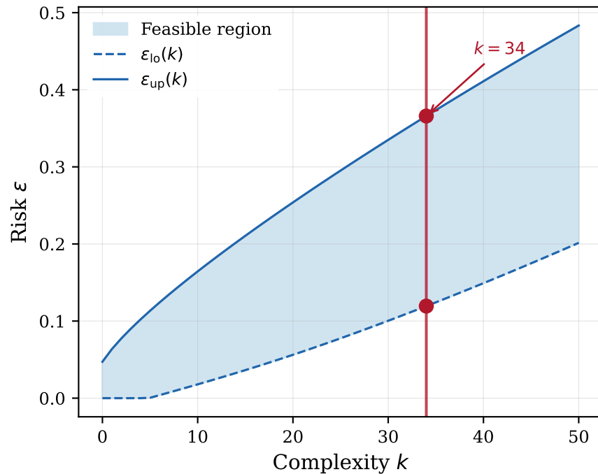
(b) Risk bounds ( N = 150, \beta = 0.01 )
