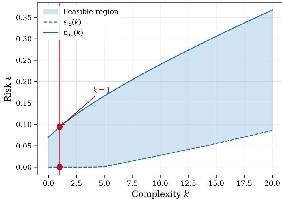
(b) Risk bounds ( N = 100 , 99\% confidence)
