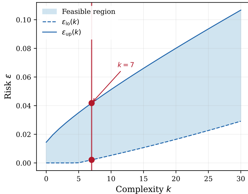
(b) Risk bounds ( N = 500 , 99\% confidence)
