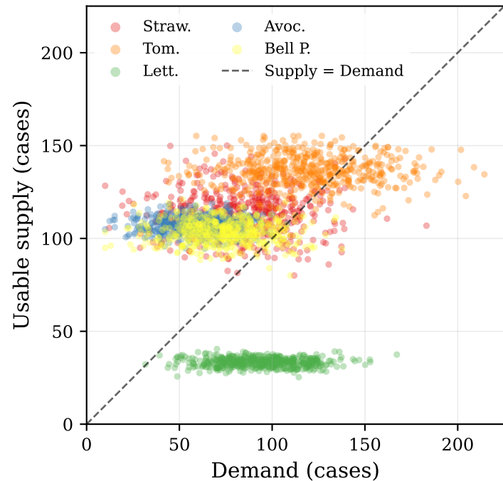
(c) Usable supply vs. demand
