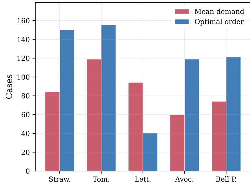
(a) Order quantities vs. mean demand
