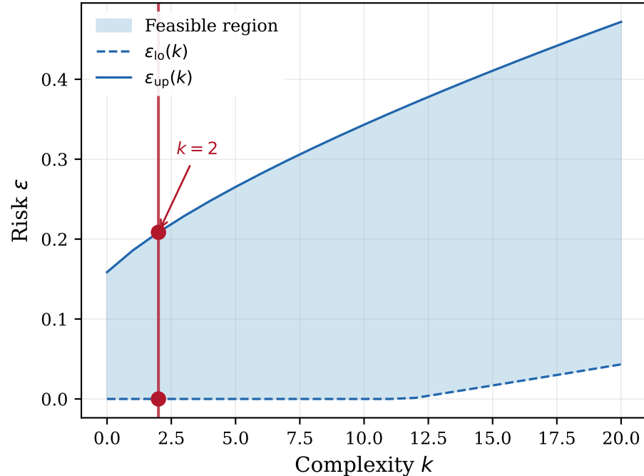
(b) Risk bounds ( N = 100, \beta = 10^{-6} )
