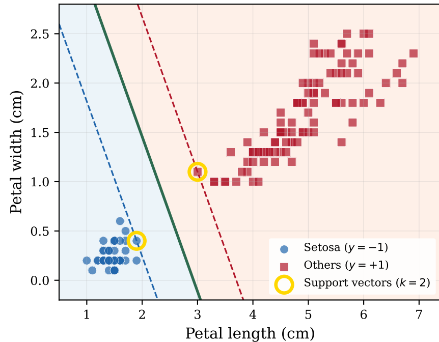
(a) SVM classification
