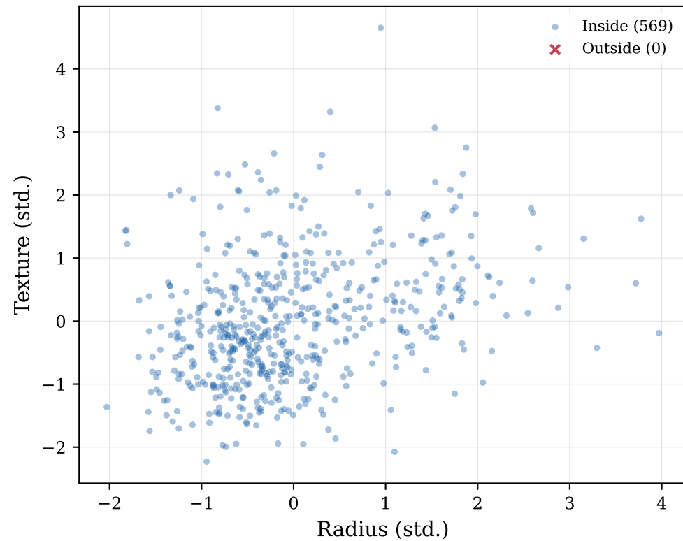
(a) Ellipsoid containment (2D projection)
