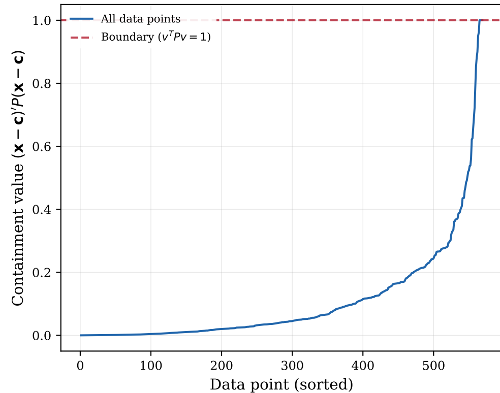
(c) Containment profile ( k = 5 , N = 569 )
