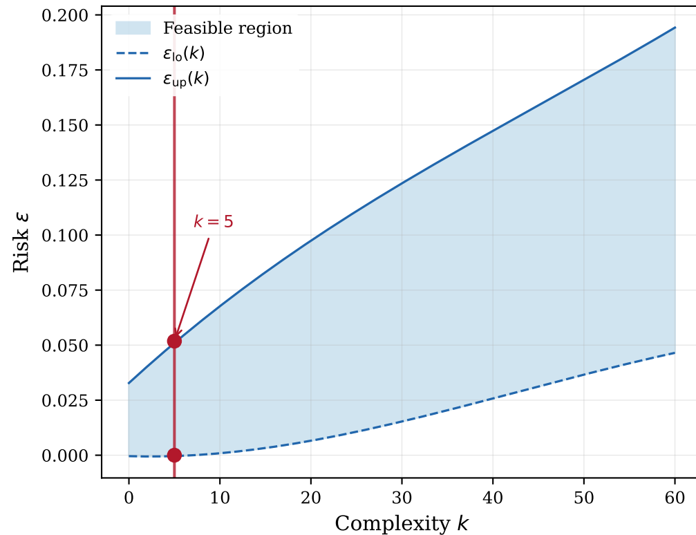
(b) Risk bounds ( N = 569 , \beta = 1e - 06 )
