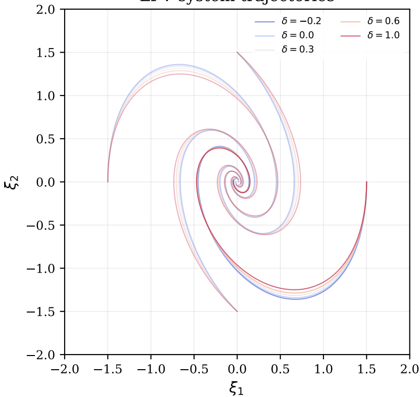
LPV system trajectories
