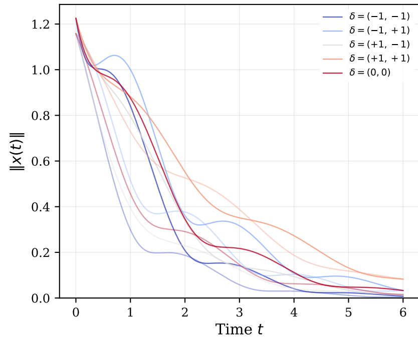
(a) Stabilising trajectories
