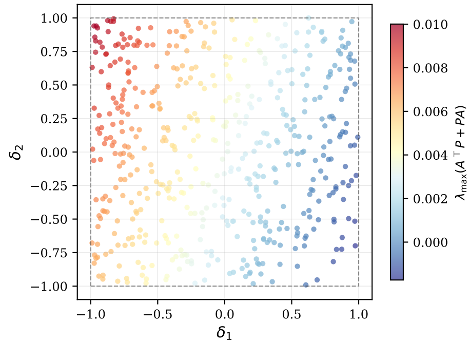
(c) Stability margin over parameter space
