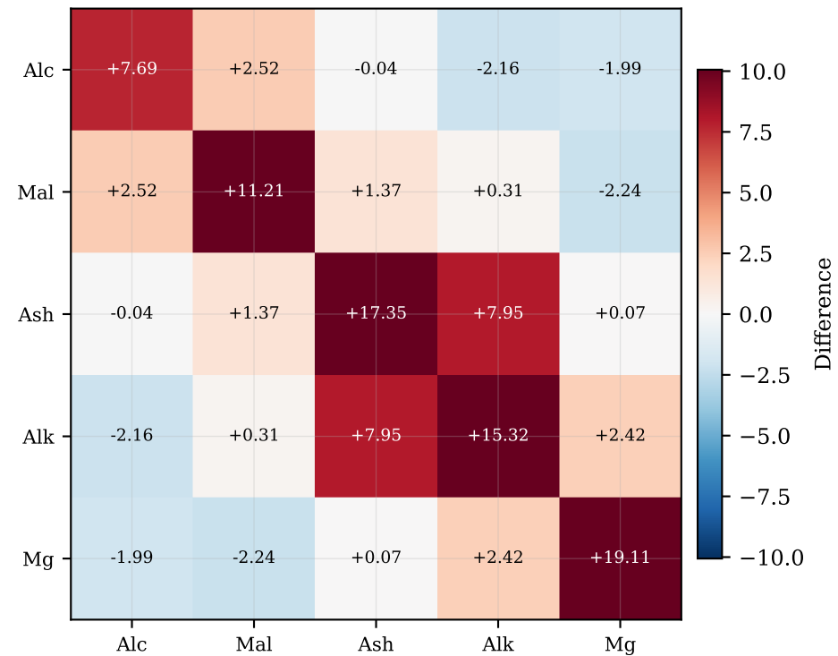
(a) \hat{\Sigma} - \Sigma_{\text{full}} (entry errors)
