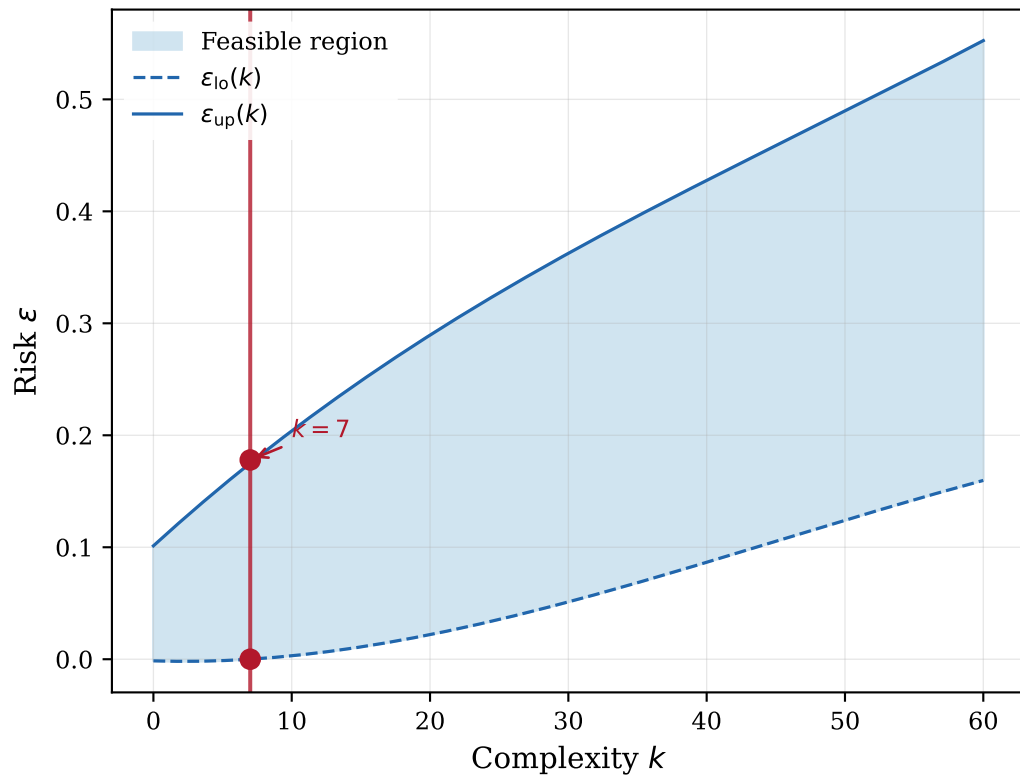
(b) Risk bounds ( N = 178 , \beta = 1e - 06 )
