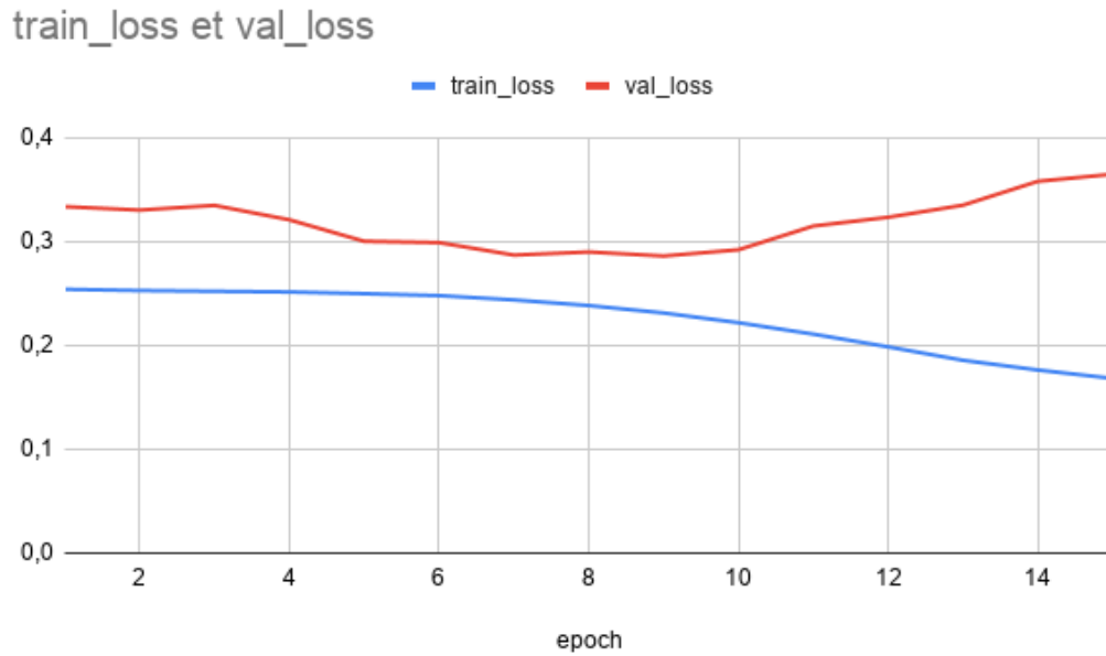
Figure 15: Training and validation loss evolution across epochs for Experiment 2.
