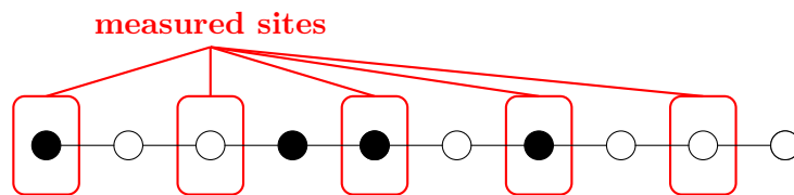
Figure 1: One-dimensional fermionic chain with local measurements applied on a finite fraction of sites.
