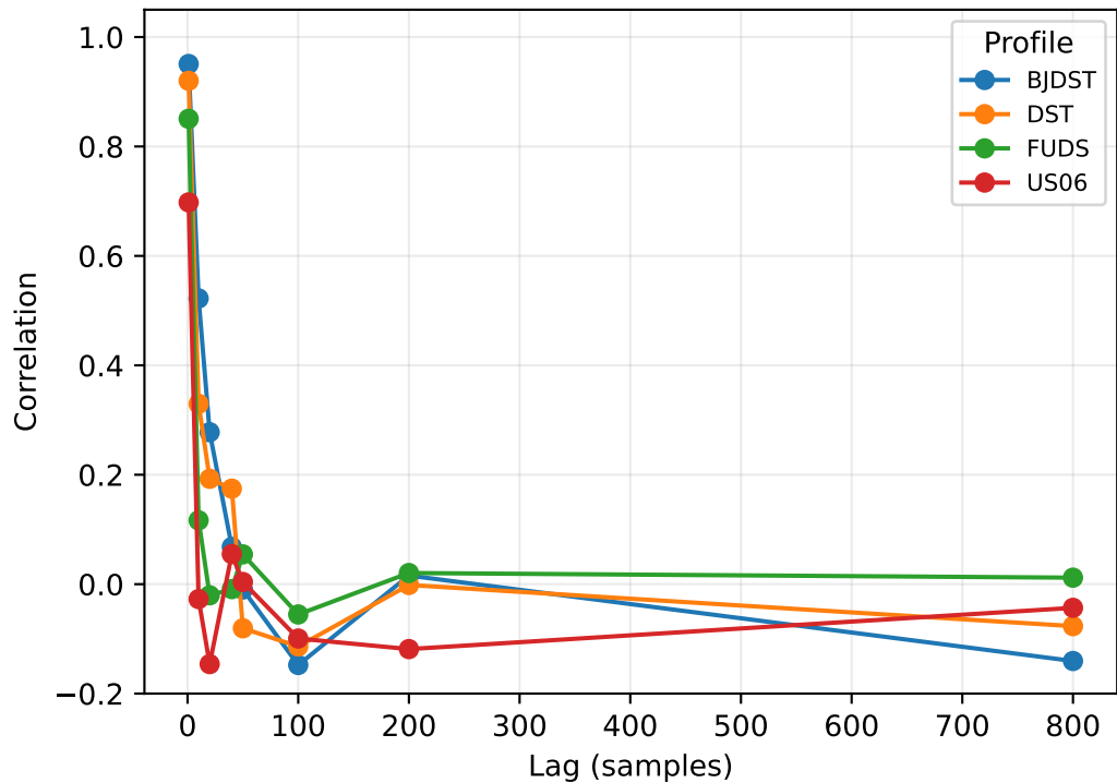
Current autocorrelation
