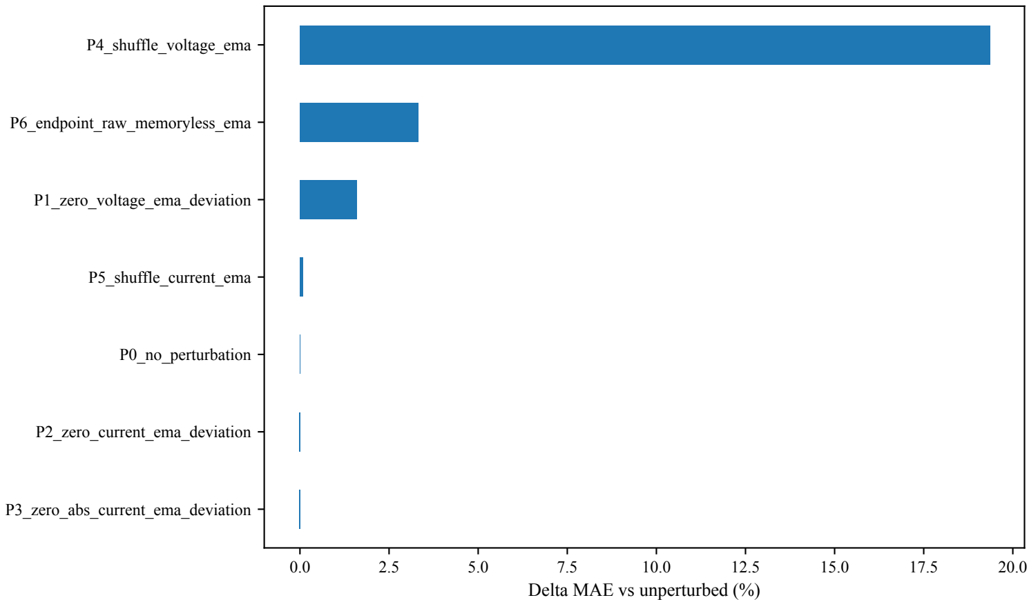
EMA Perturbation Importance
