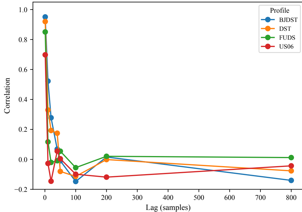
Current autocorrelation
