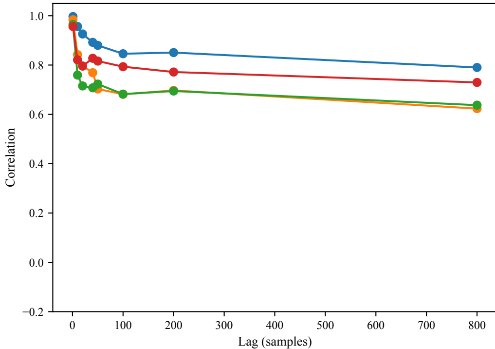
Voltage autocorrelation
