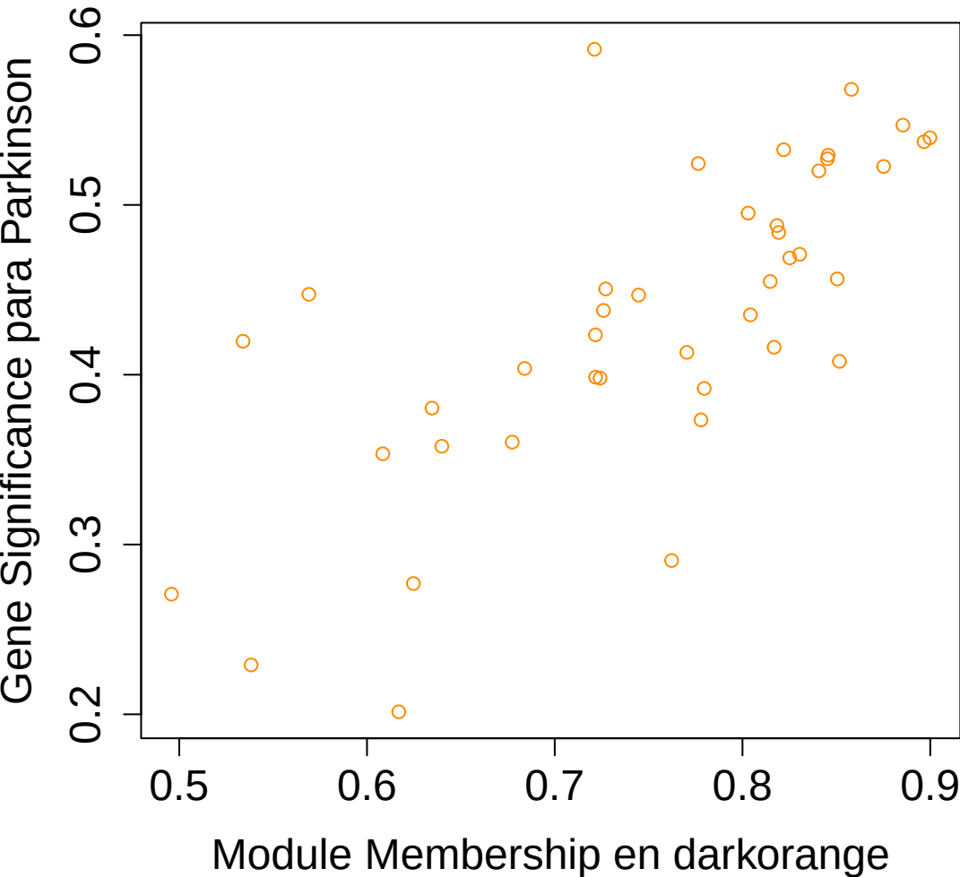
GS vs MM – módulo darkorange cor=0.72, p=7.7e-
