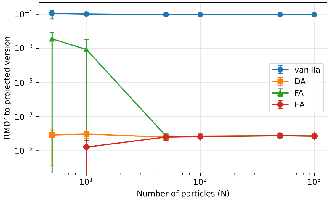
RMD 2 to E ^ G at end of training — NN, matrix setup, arbitrary teacher (SI init)
