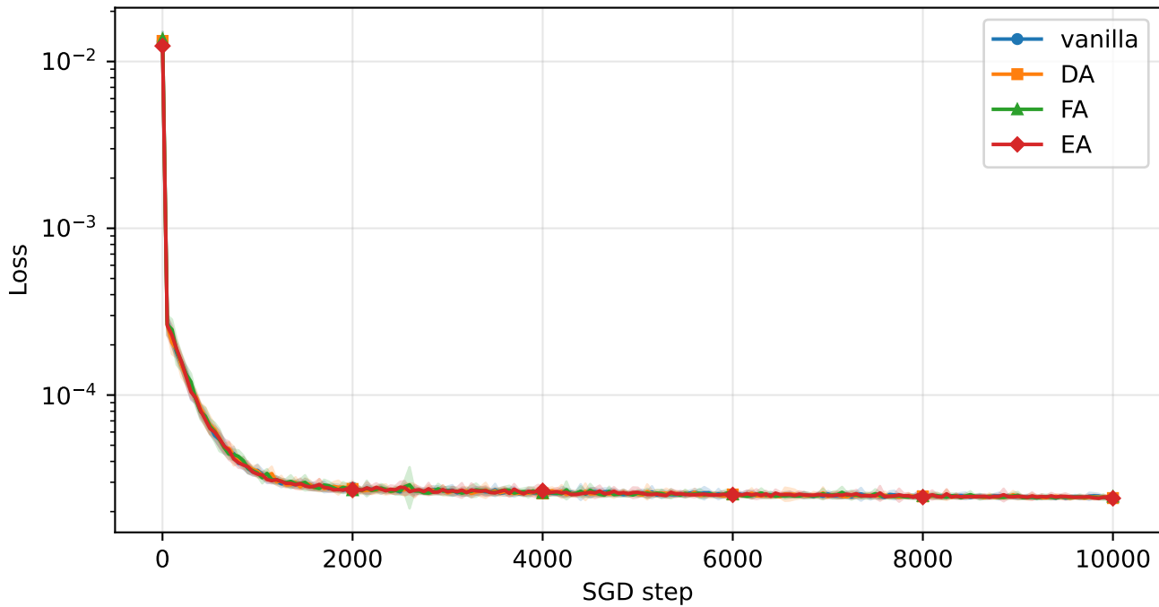
Training loss vs SGD step — NN, matrix setup, WI teacher (SI init, N=500)
