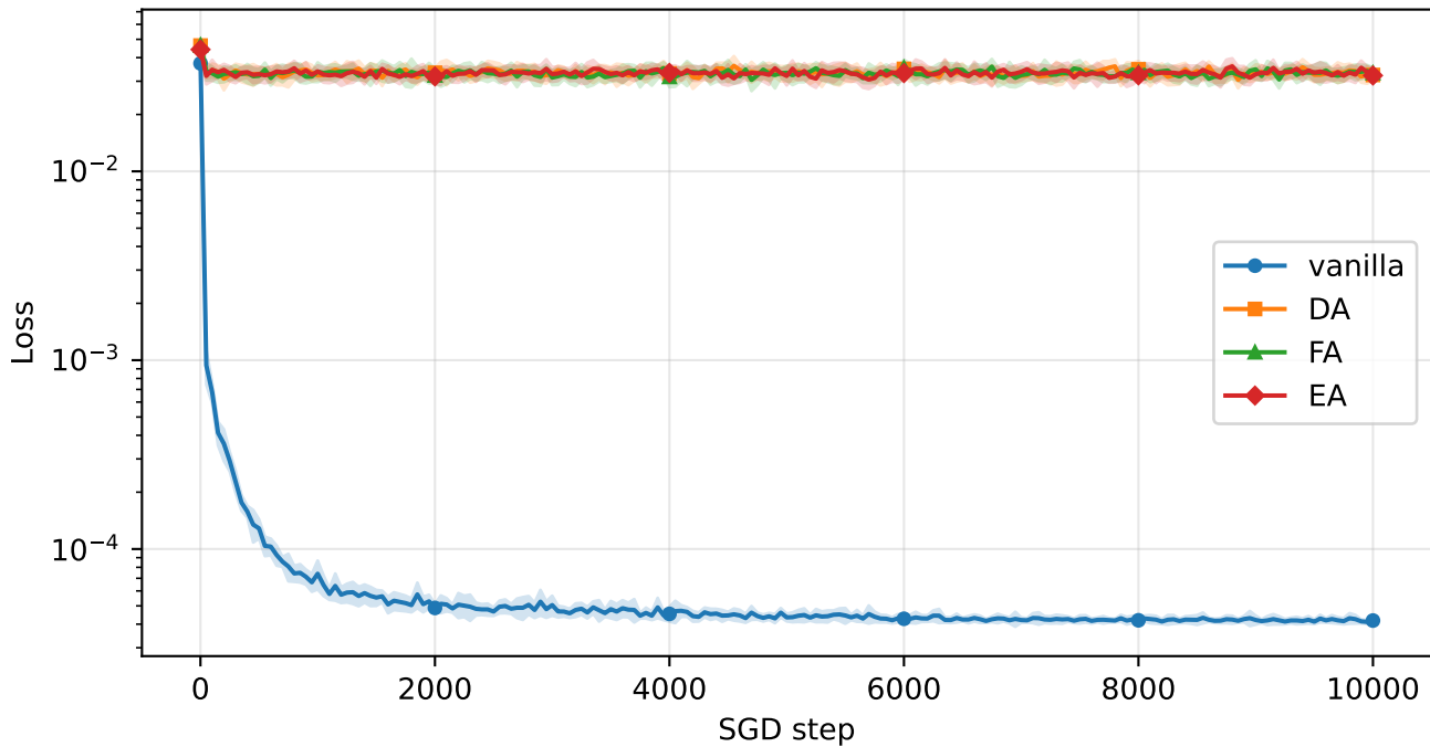
Training loss vs SGD step — NN, matrix setup, arbitrary teacher (SI init, N=500)
