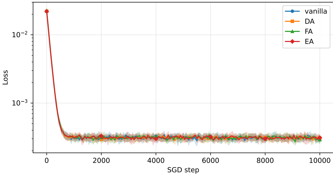
Training loss vs SGD step — NN, uv setup, WI teacher (SI init, N=500)
