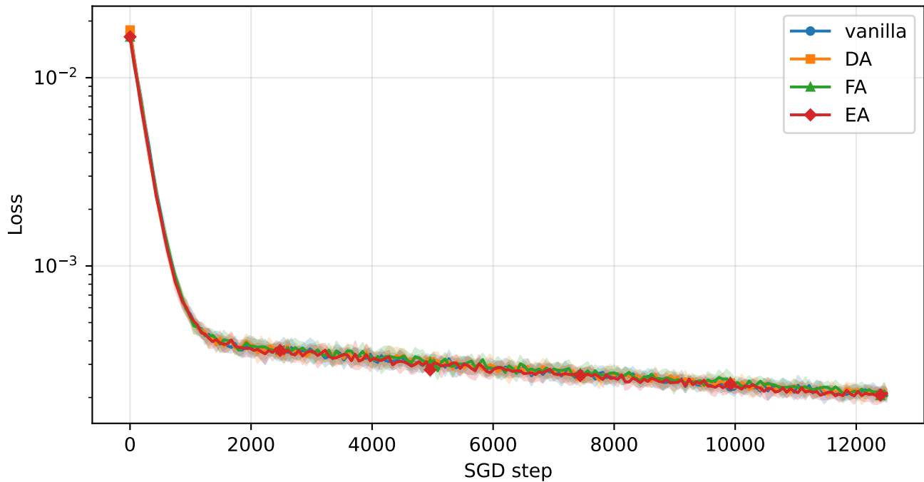
Training loss vs SGD step — ResNet, matrix setup, WI teacher (SI init, M=5, L=500)
