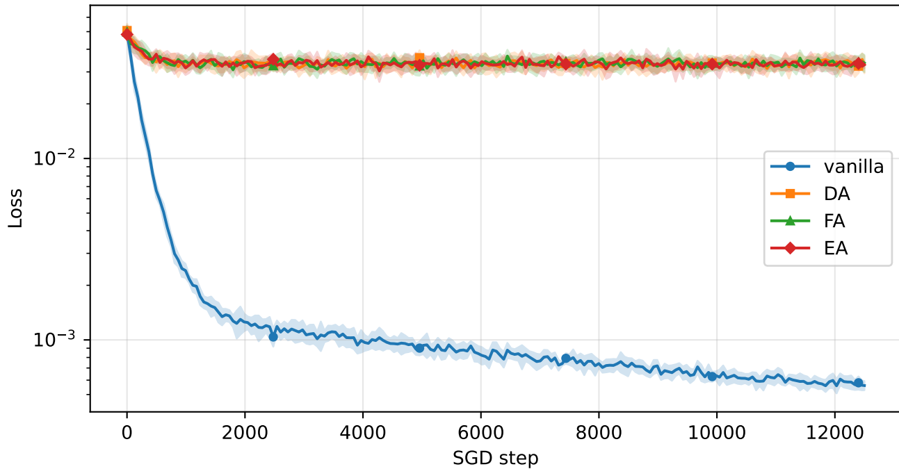
Training loss vs SGD step — ResNet, matrix setup, arbitrary teacher (SI init, M=5, L=500)
