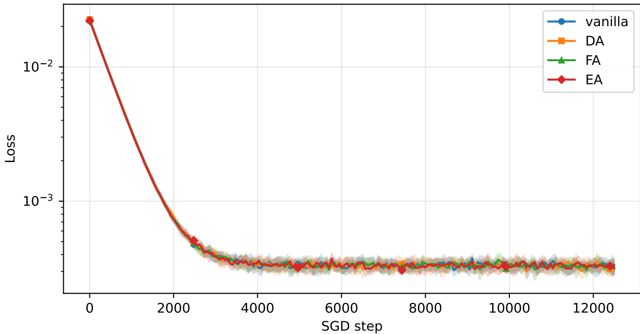
Training loss vs SGD step — ResNet, uv setup, WI teacher (SI init, M=5, L=500)
