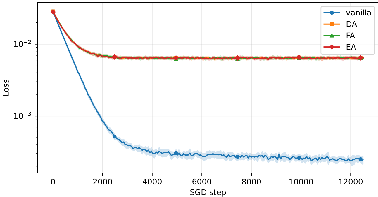
Training loss vs SGD step — ResNet, uv setup, arbitrary teacher (SI init, M=5, L=500)
