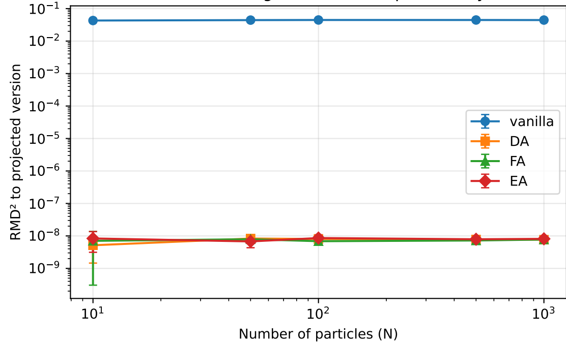
RMD 2 to E ^ G at end of training — NN, uv setup, arbitrary teacher (SI init)
