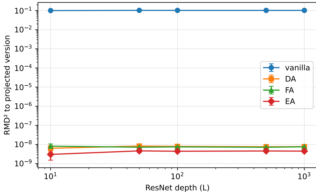
RMD 2 to E ^ G at end of training — ResNet, matrix setup, arbitrary teacher (SI init)
