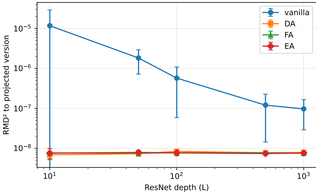
RMD 2 to E G at end of training — ResNet, uv setup, WI teacher (SI init)
