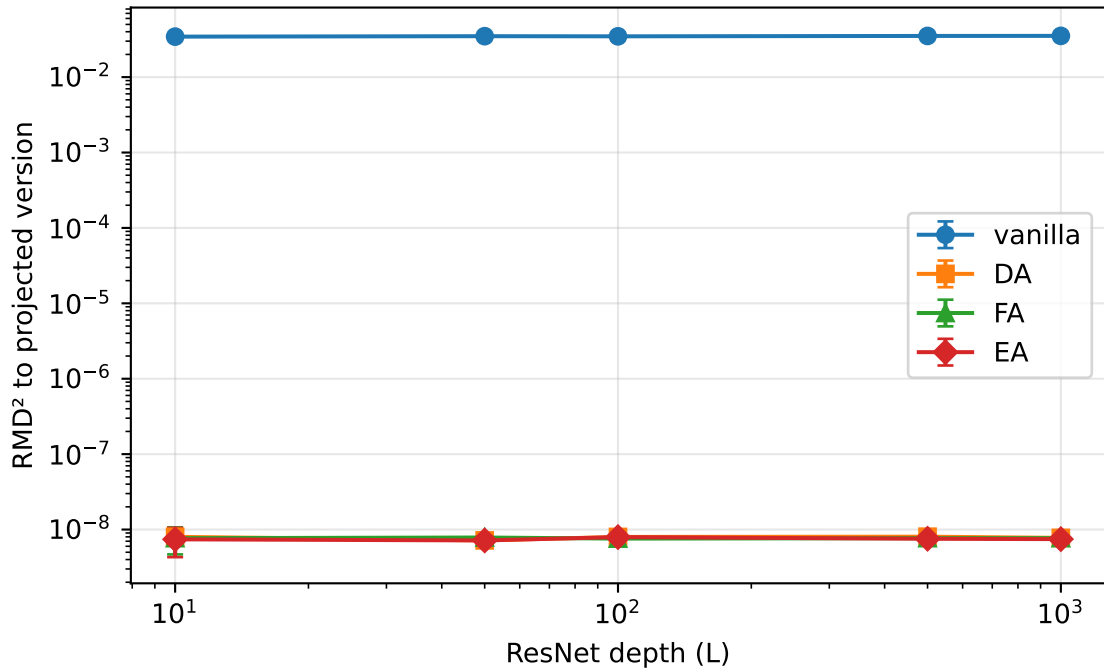
RMD 2 to E ^ G at end of training — ResNet, uv setup, arbitrary teacher (SI init)
