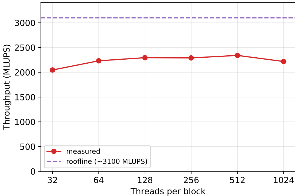
CUDA block-size sweep ( 1024^2 , SoA)
