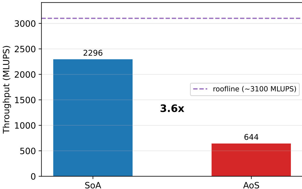
CUDA: SoA vs AoS — coalescing gives ~3.6x
