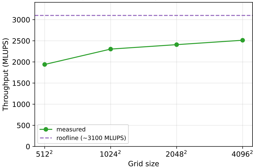
CUDA problem-size sweep (SoA, block=256)
