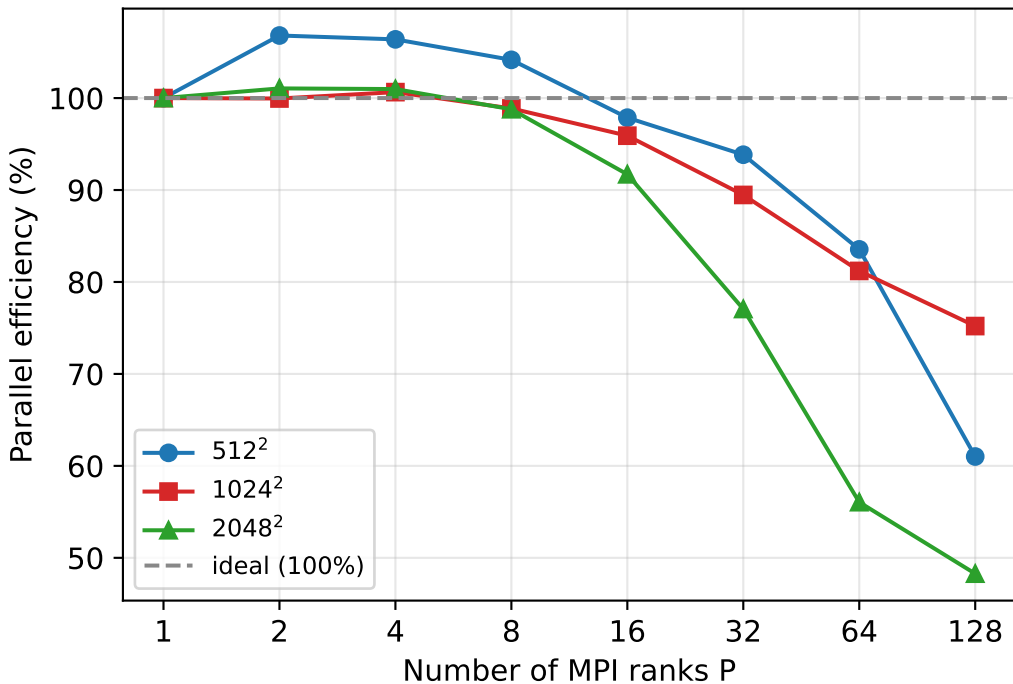
MPI strong scaling: efficiency E(P)
