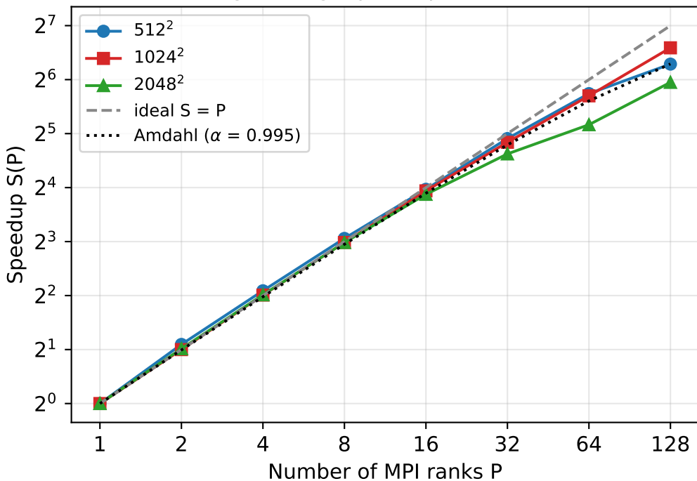
MPI strong scaling: speedup vs ideal / Amdahl
