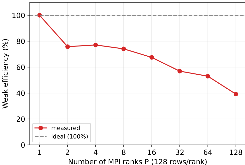
MPI weak scaling: 100% -> 39% (1 -> 128 ranks)
