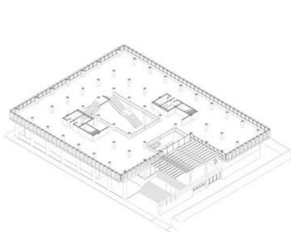
Isometric 1st Floor
