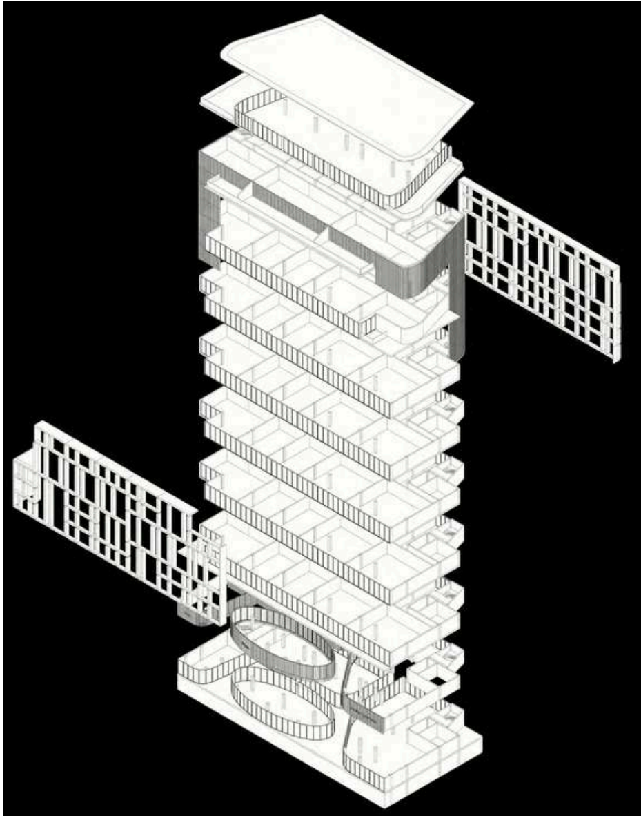
Exploded Axonometric View
