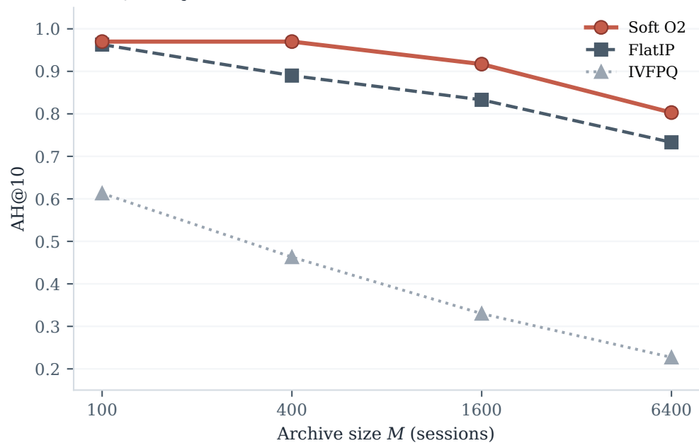
(a) Quality vs scale (DISC exact)
