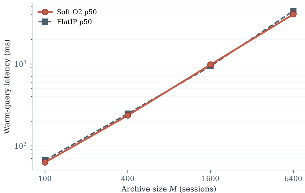
(b) Latency vs scale
