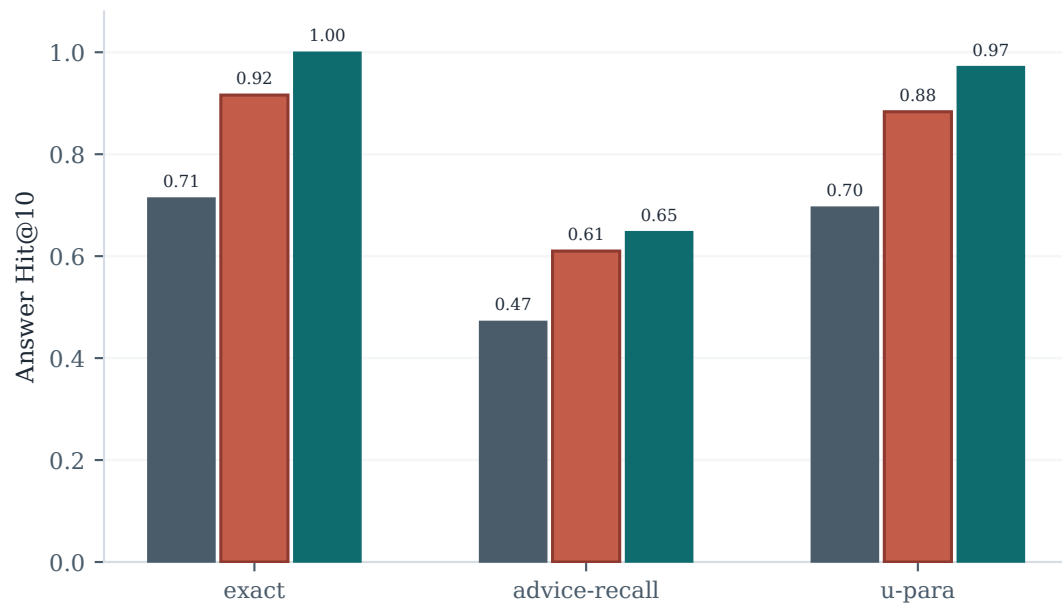
(a) LegalEp-DISC AH@10
