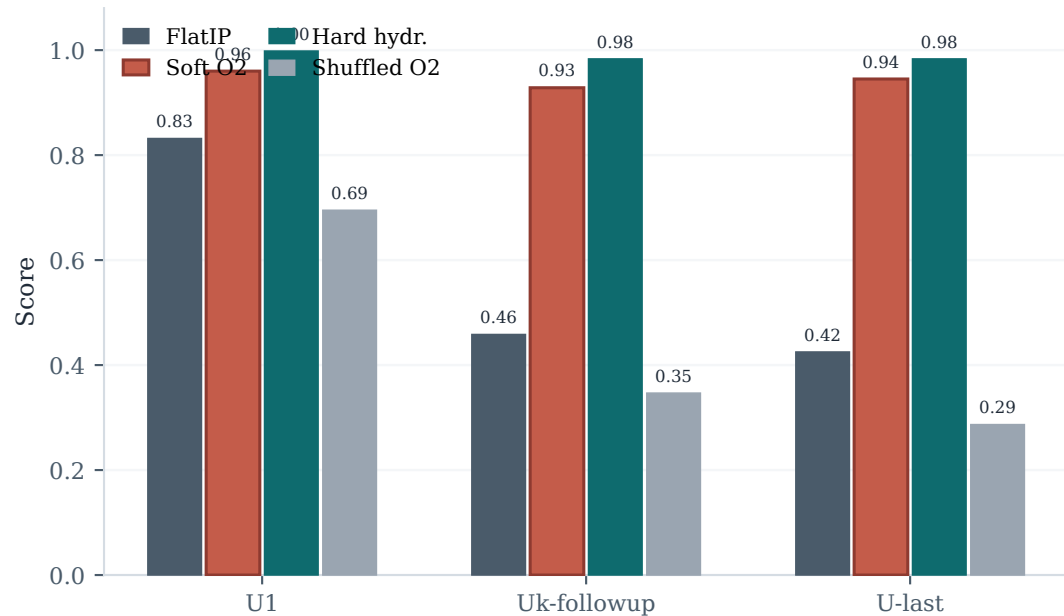
(a) Answer Hit@10
