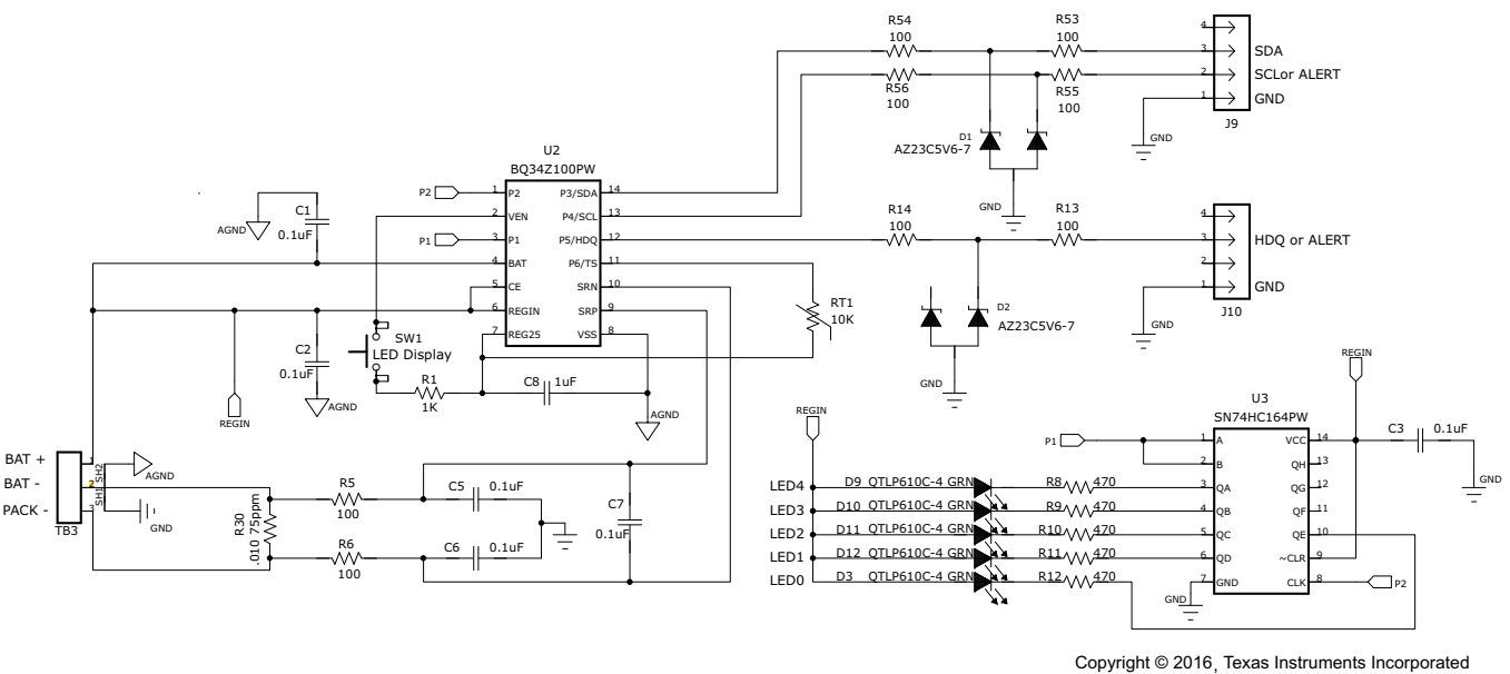
Figure 8-2. 1-Cell Li-ion and 5-LED Display
