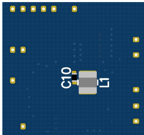
Figure 54. Board Layout- Bottom
