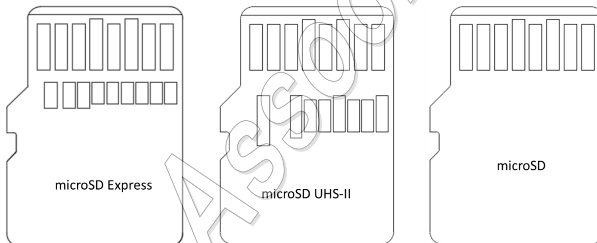
Figure L-6 : microSD Card Simplified Dimensions Pads side
