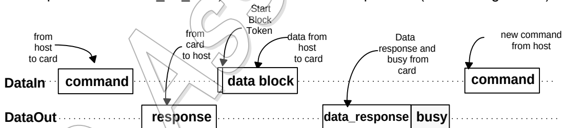
Figure 7-6 : Single Block Write Operation
