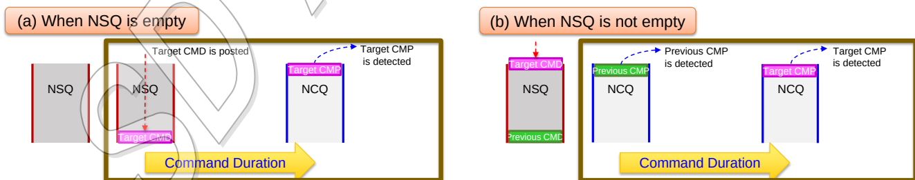
Figure 8-20 : Definition of Command Duration in the SD Express Speed Class
