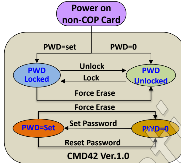
Figure 4.3.7-1 : Simplified Non-COP Card State Diagram
