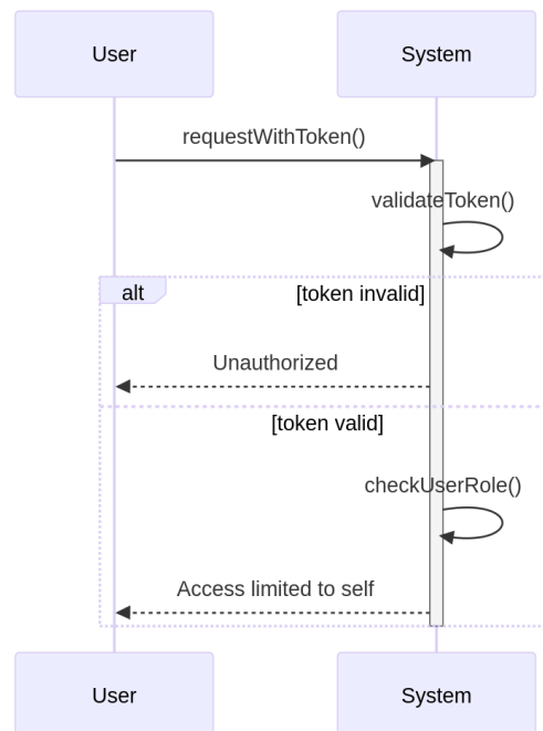
Figure 3.27: User authorization sequence diagram
