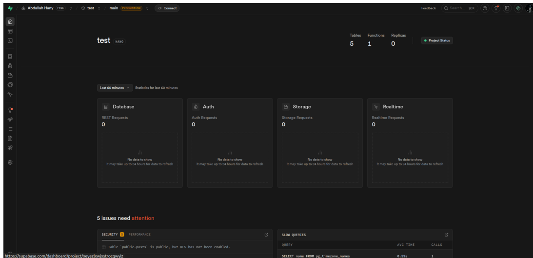
Figure 2.5: Supabase console
