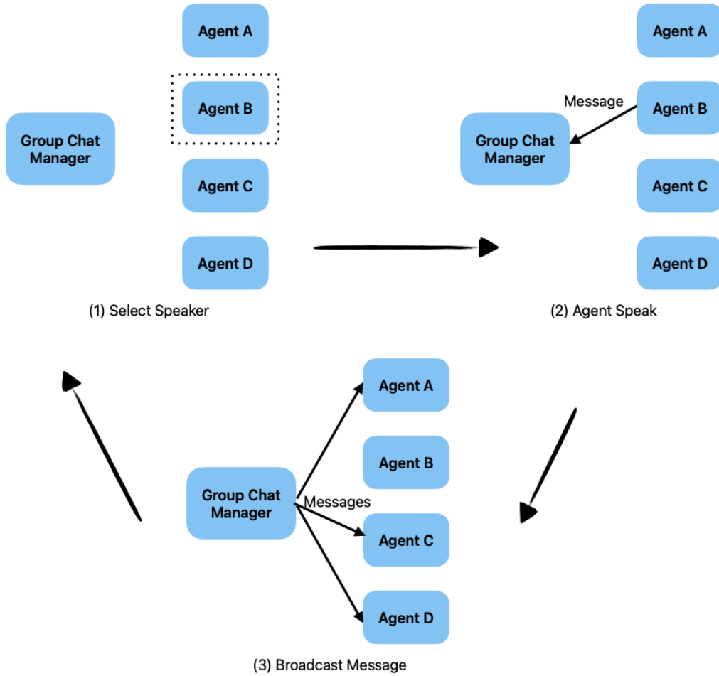
Figure 2.16: Group conversation pattern
