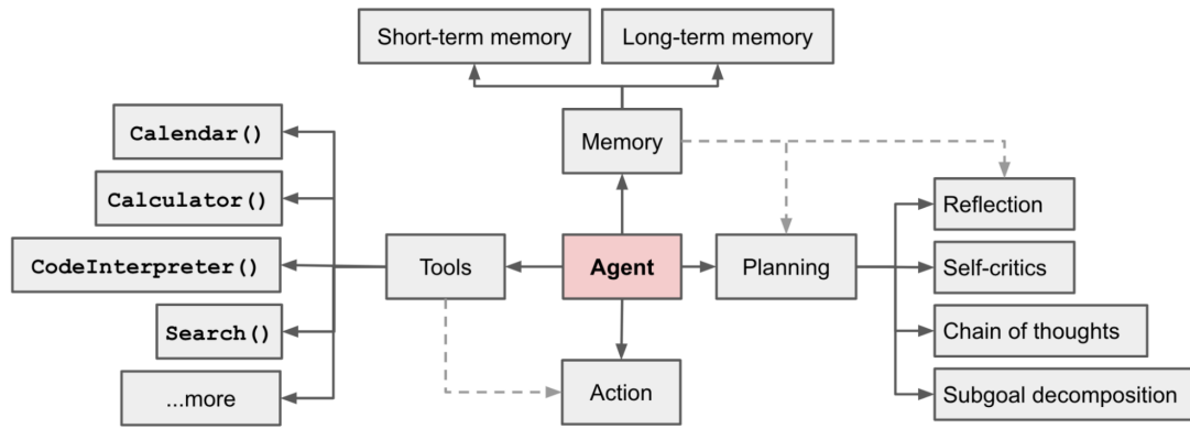
Figure 2.12: AI Agent Tool-Calling Architecture.
