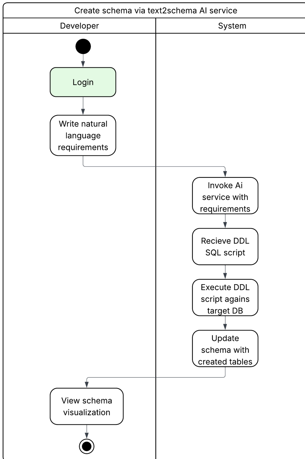
Figure 3.17: Create SQL schema via AI activity diagram
