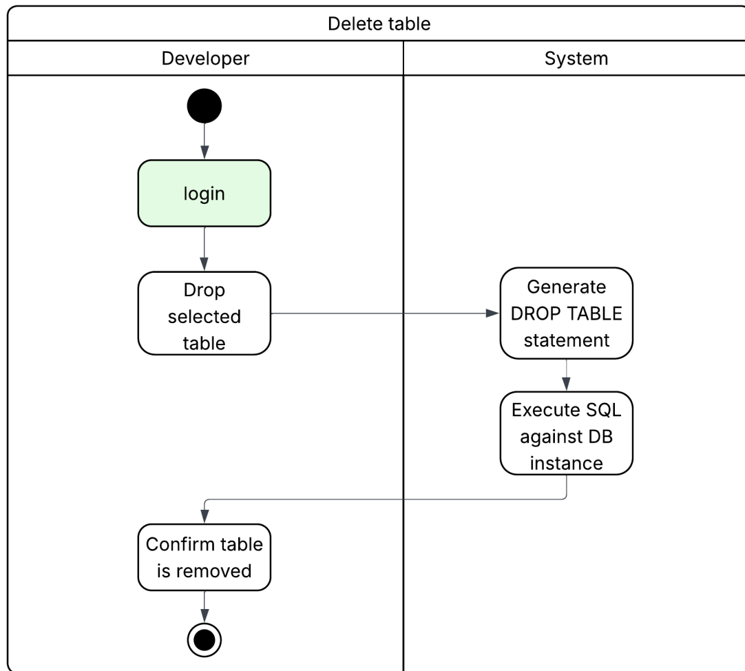
Figure 3.8: Delete SQL table activity diagram
