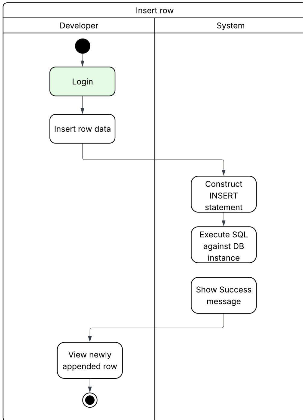
Figure 3.13: Insert SQL rows activity diagram
