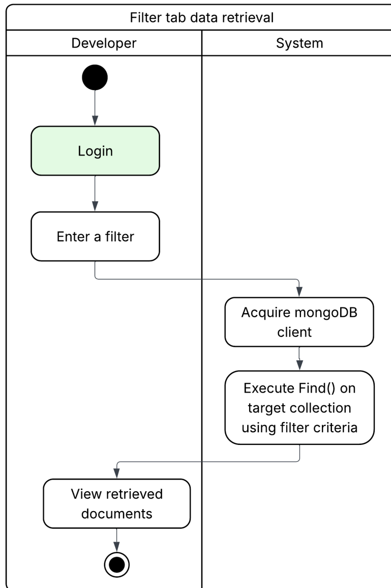
Figure 3.25: Data retrieval via NoSQL filter activity diagram
