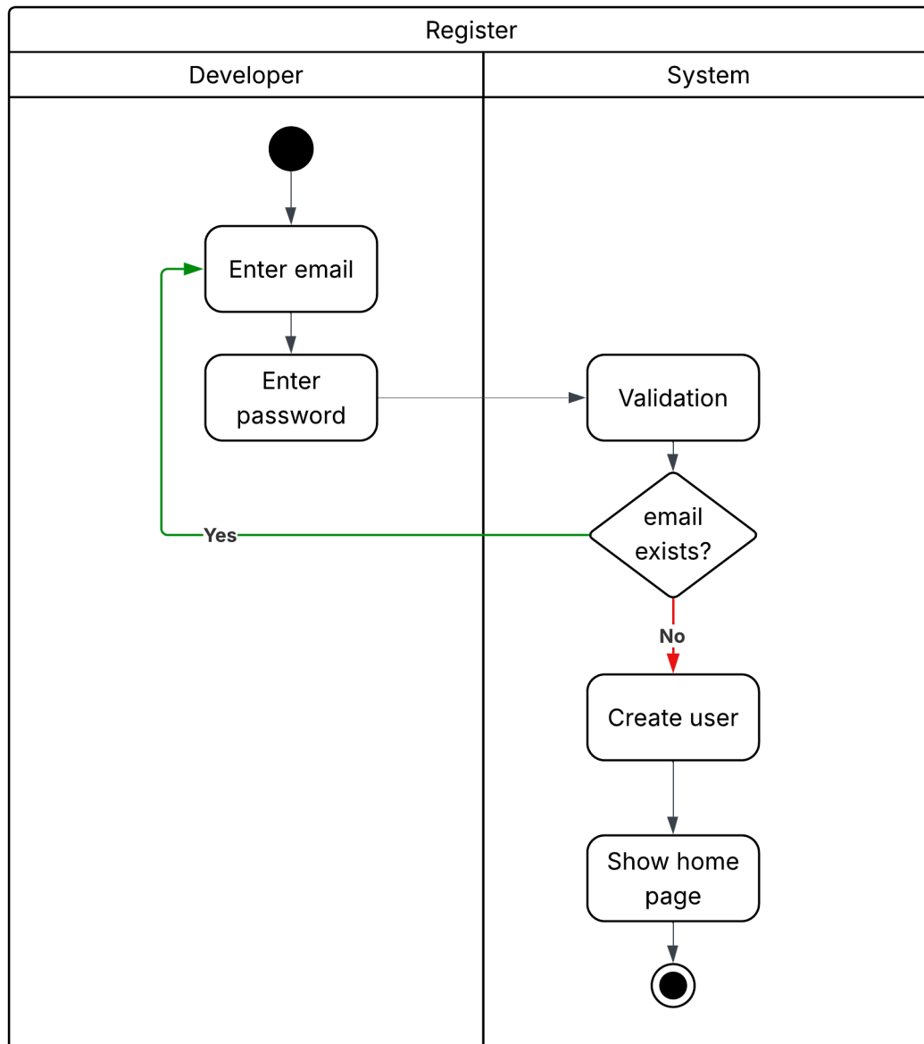
Figure 3.1: Register activity diagram
