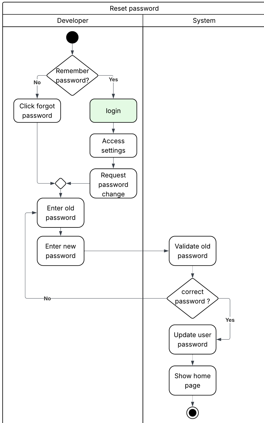
Figure 3.4: Reset password activity diagram
