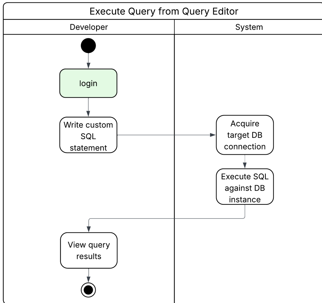
Figure 3.16: Execute SQL query activity diagram
