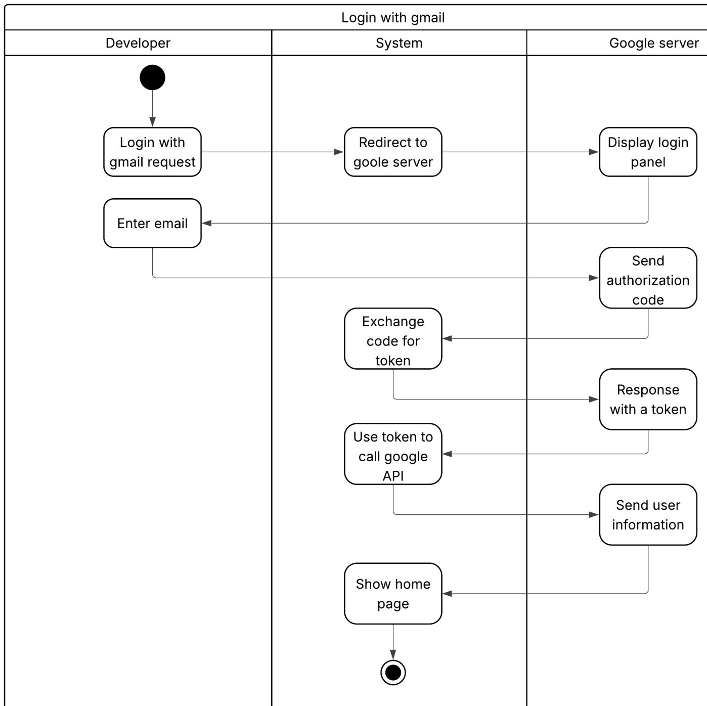
Figure 3.3: Login with g-mail activity diagram
