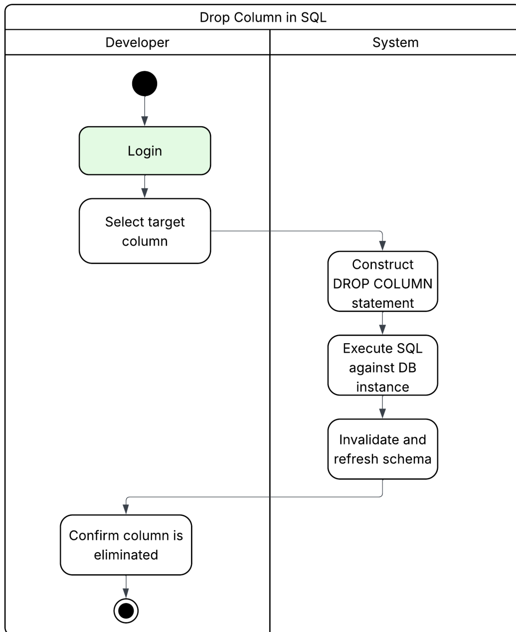
Figure 3.10: Drop SQL column activity diagram
