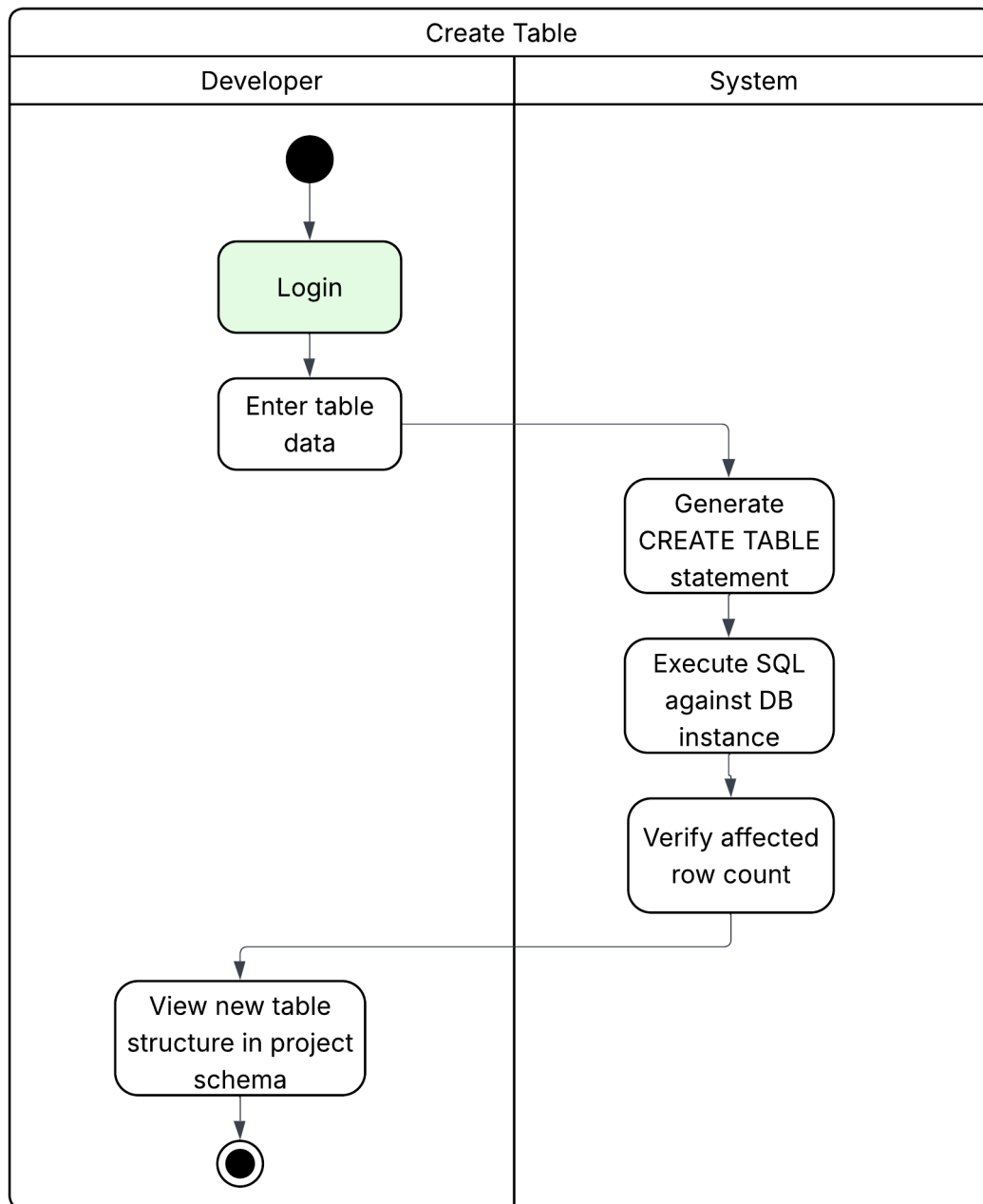
Figure 3.7: Create SQL table activity diagram
