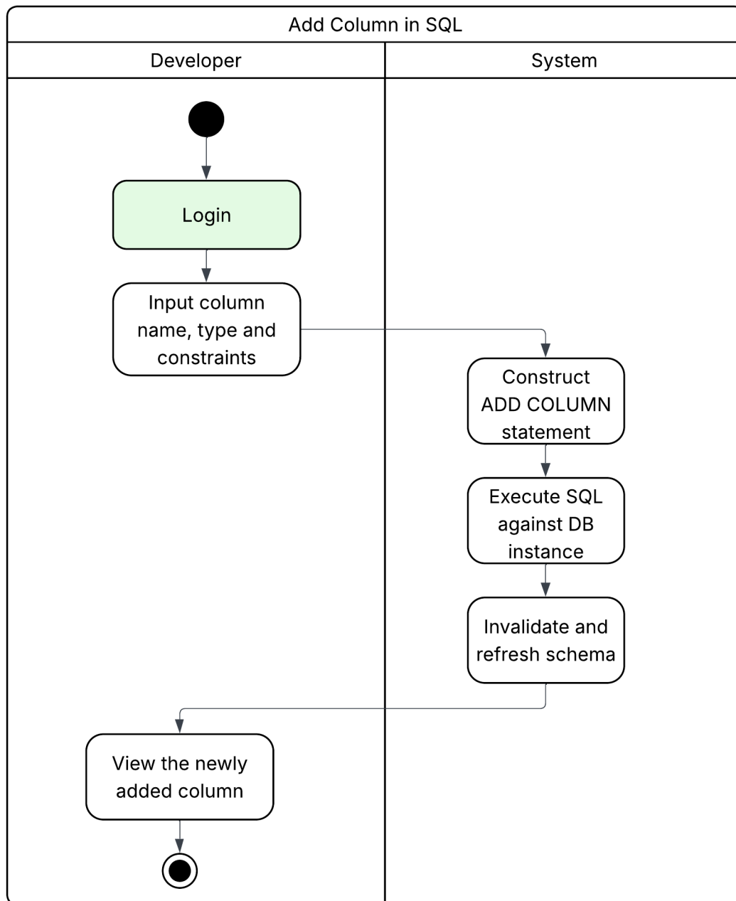
Figure 3.9: Add SQL column activity diagram
