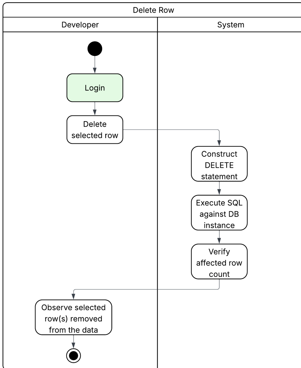
Figure 3.14: Delete SQL rows activity diagram
