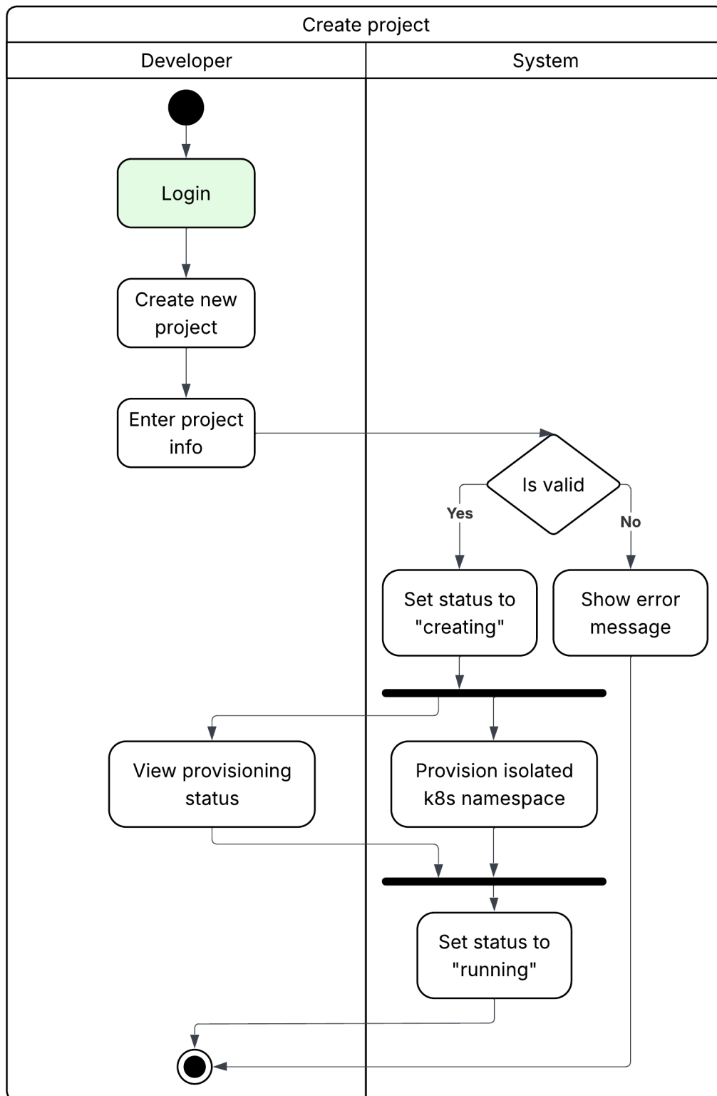
Figure 3.5: Create project activity diagram
