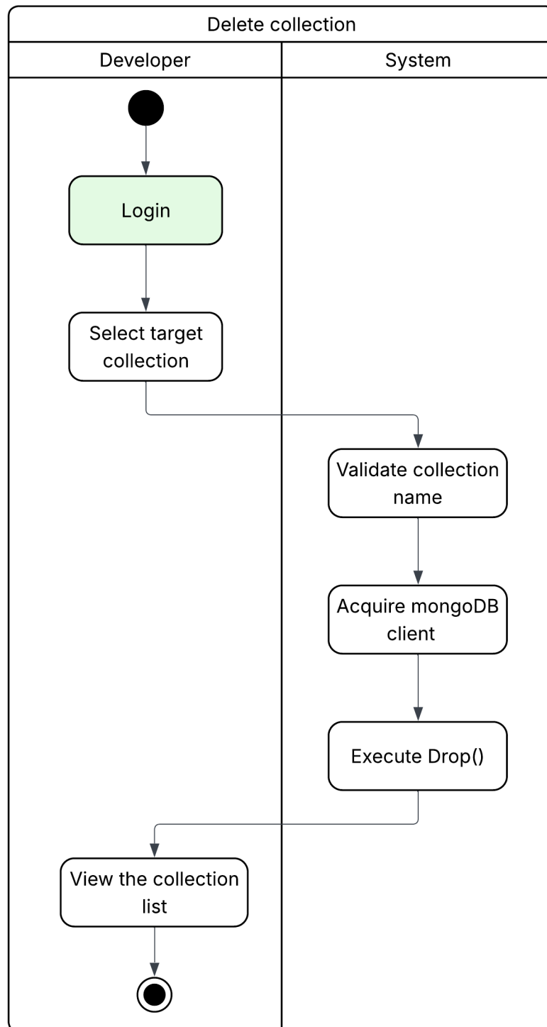
Figure 3.19: Delete NoSQL collection activity diagram
