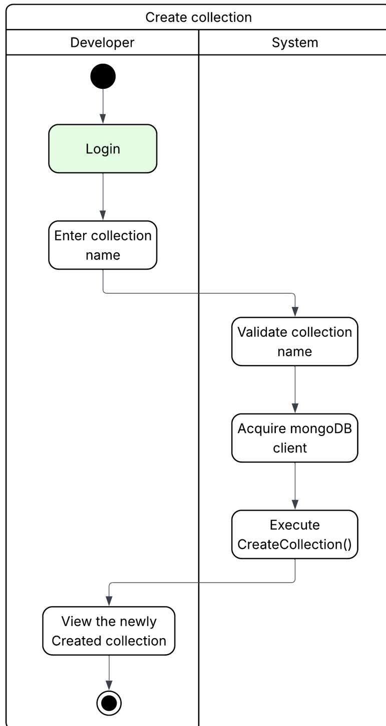
Figure 3.18: Create NoSQL collection activity diagram
