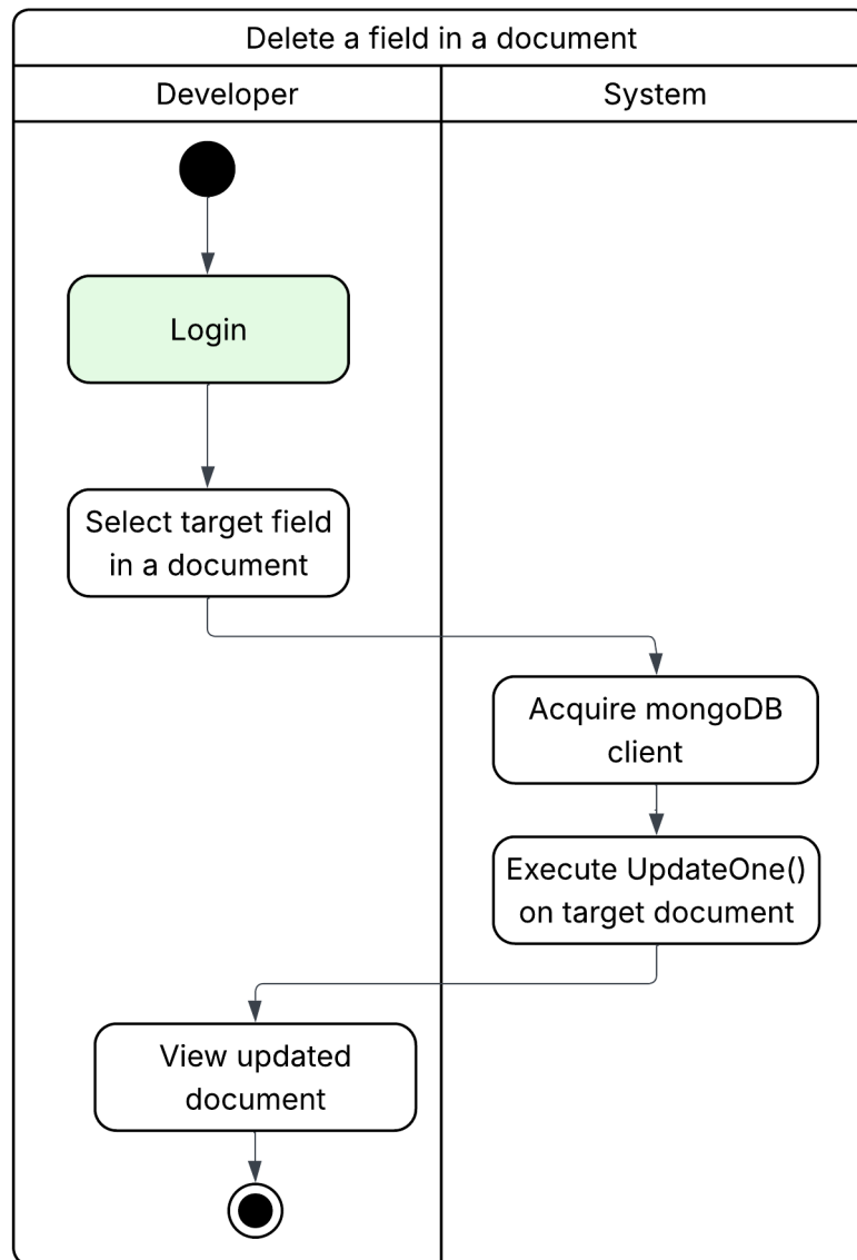
Figure 3.23: Delete a NoSQL field in a document activity diagram
