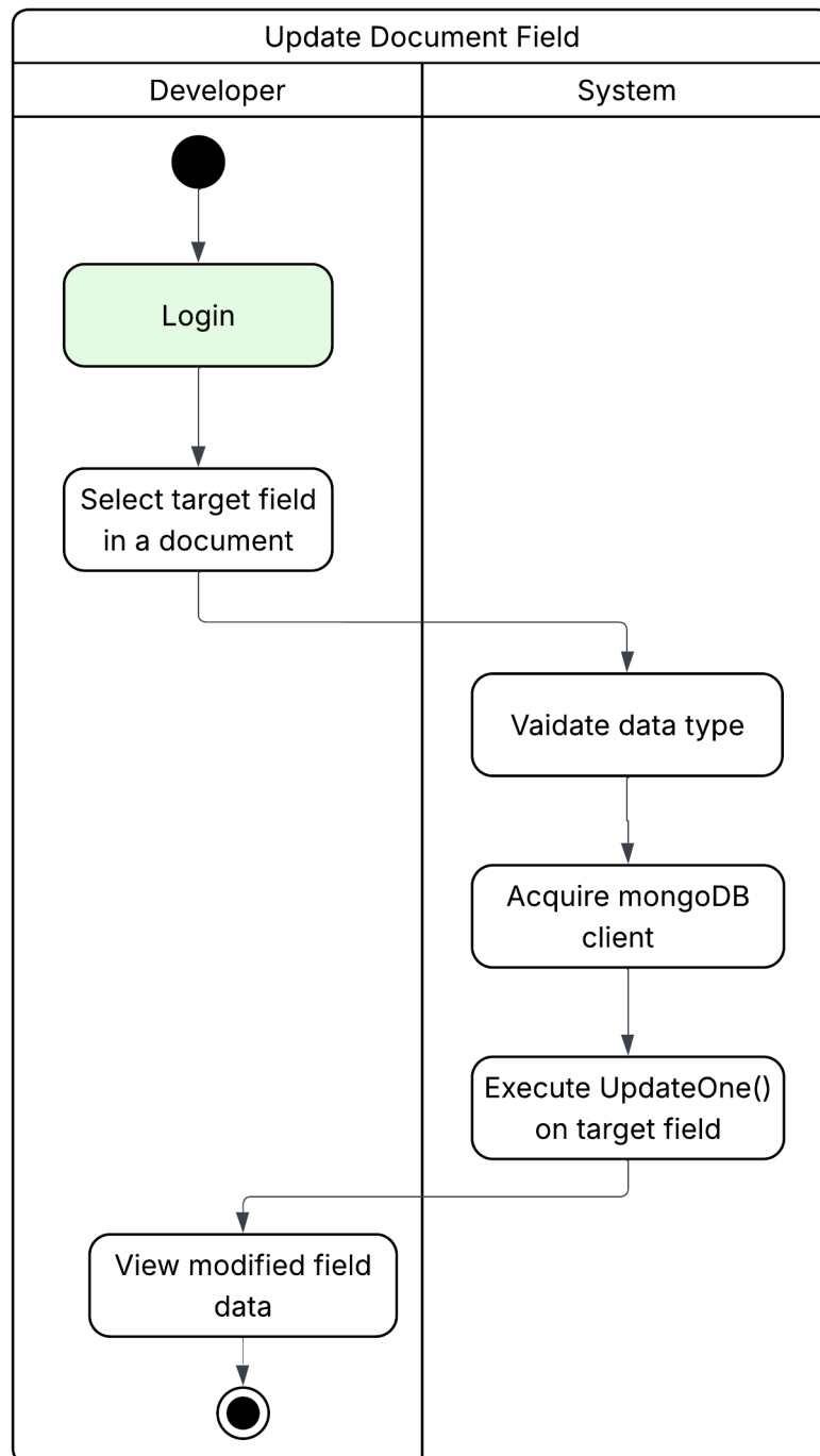
Figure 3.24: Update a NoSQL field in a document activity diagram
