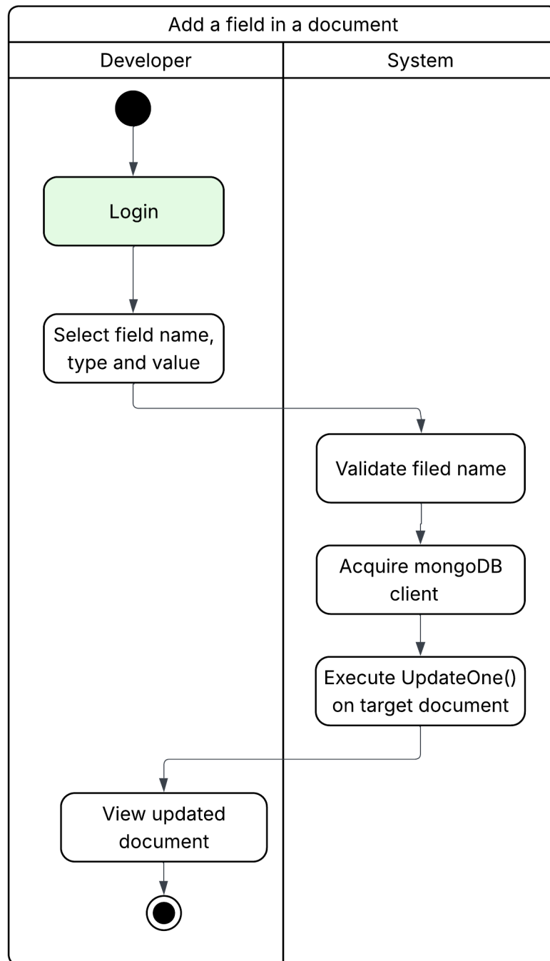
Figure 3.22: Add a NoSQL field in a document activity diagram
