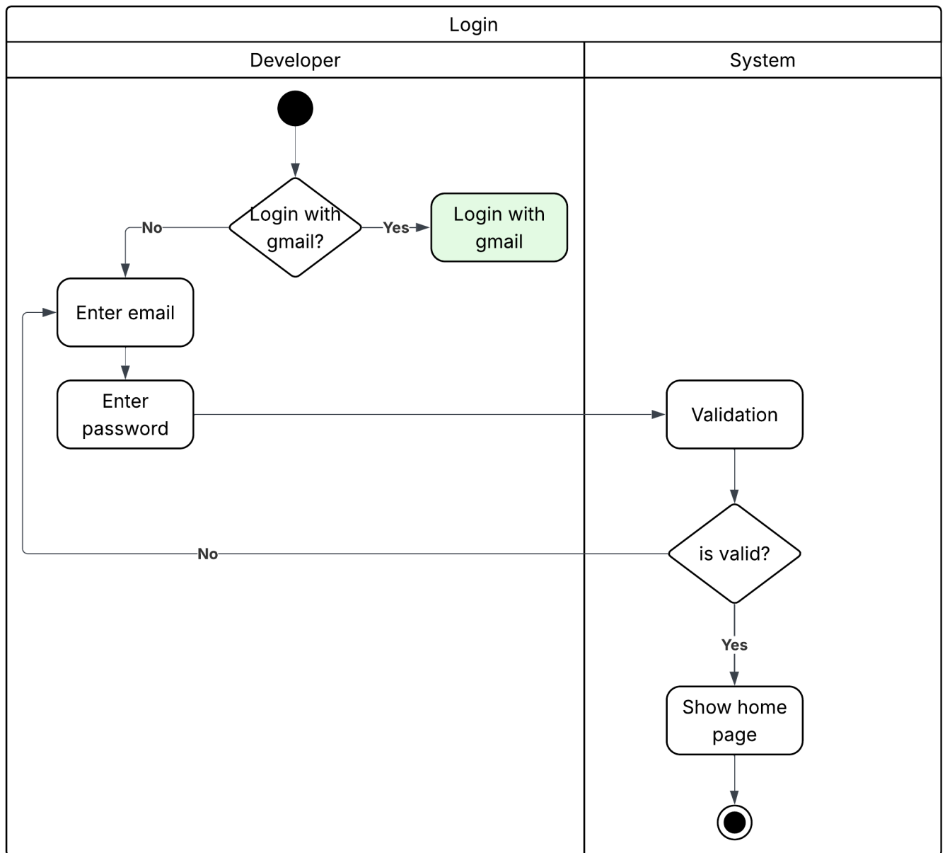
Figure 3.2: Login activity diagram
