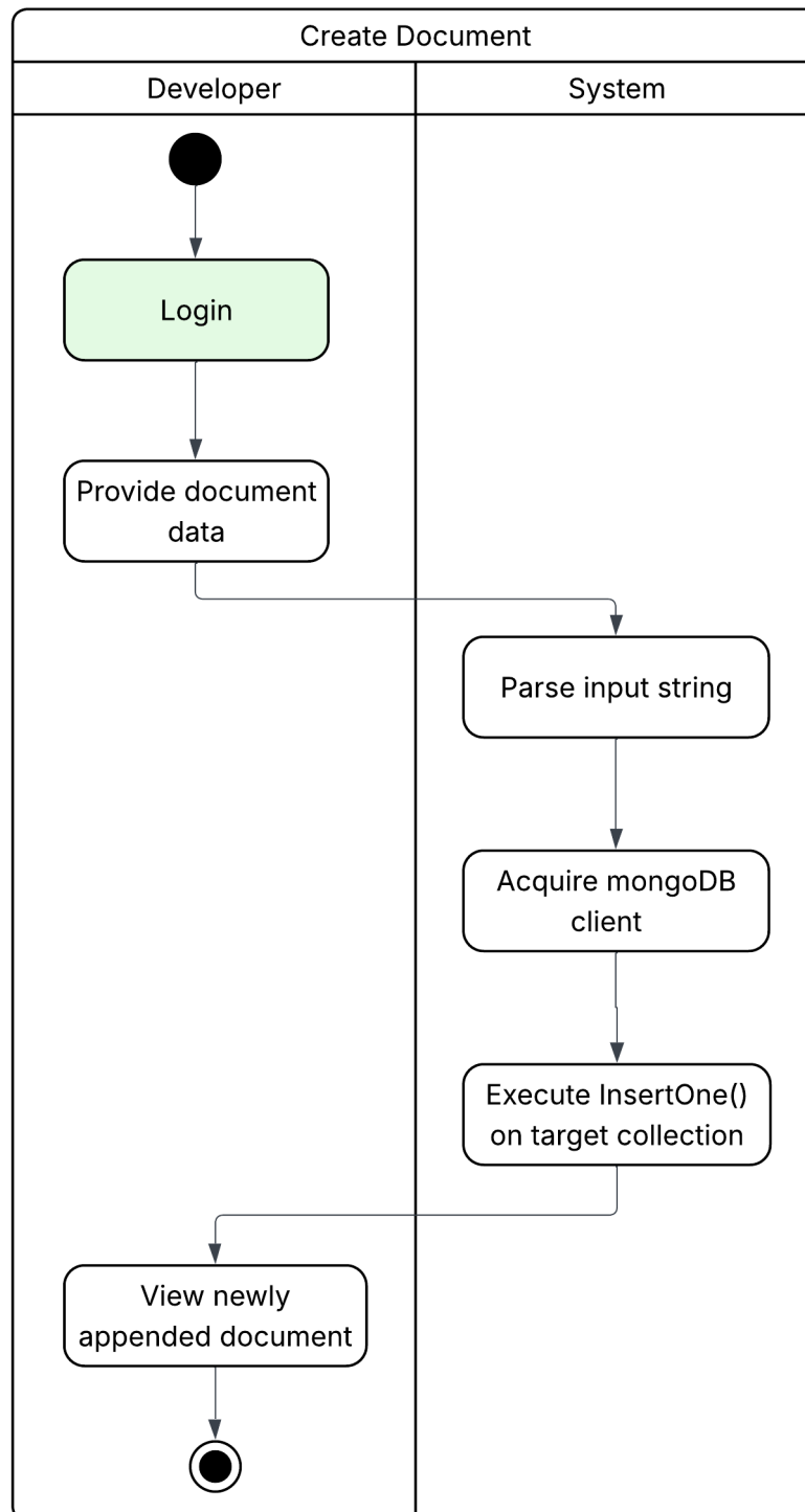
Figure 3.20: Create NoSQL document activity diagram
