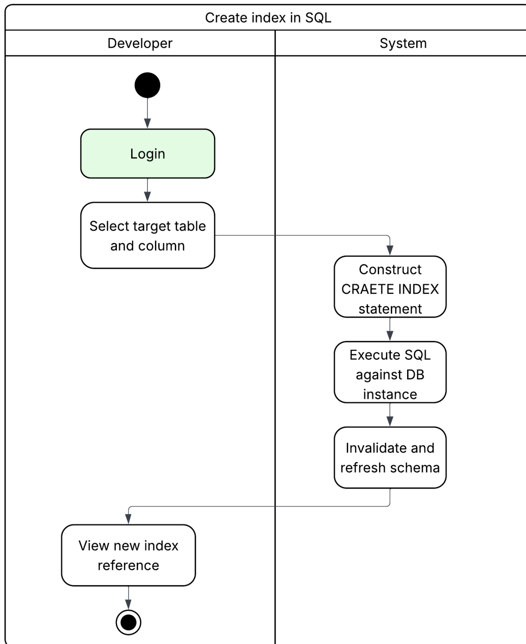
Figure 3.11: Create SQL index activity diagram
