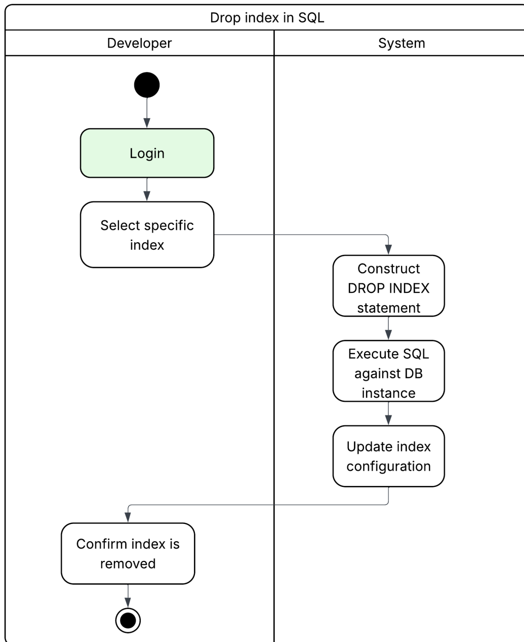
Figure 3.12: Drop SQL index activity diagram
