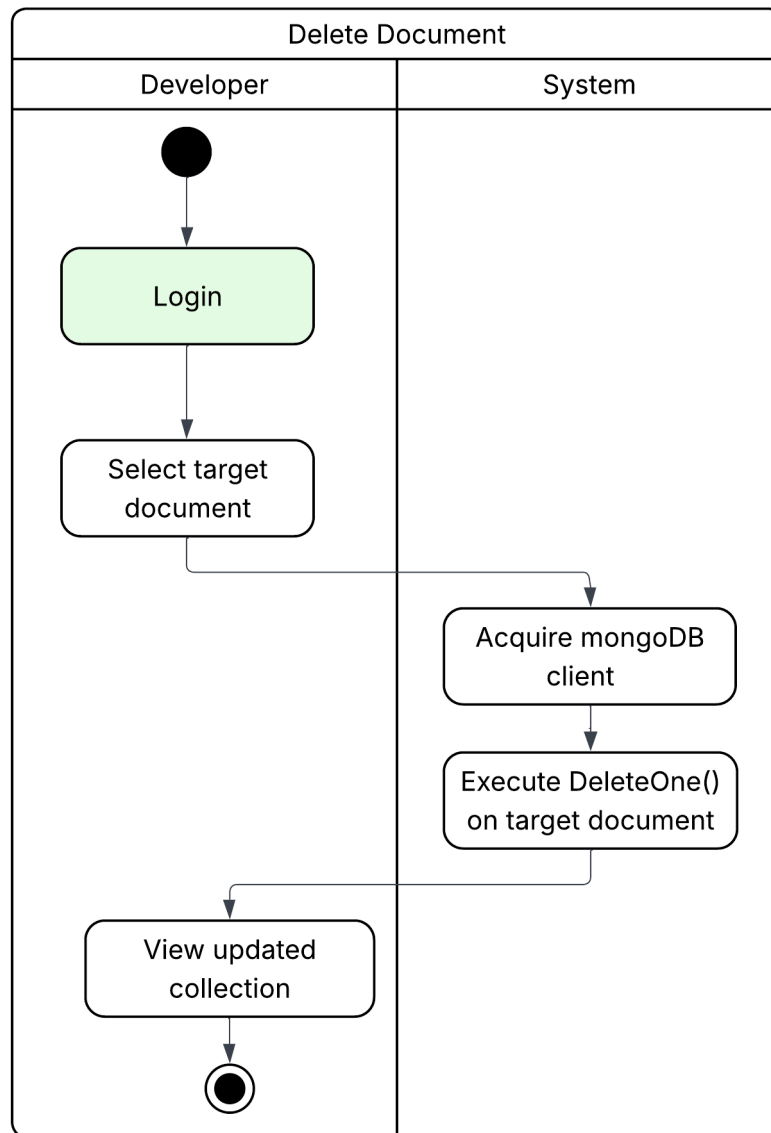
Figure 3.21: Delete NoSQL document activity diagram
