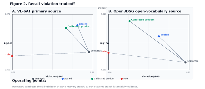
Figure 2: Recall-violation tradeoff. Lower Violation@100 and higher R@100 are better. Open3DSG is reported on the full-validation recovery branch; 533/548 and historical 377/388 vs R2 388/388 branches are sensitivity evidence only. The plotted soft operating point is the calibrated product; Table 4 compares fusion forms.
