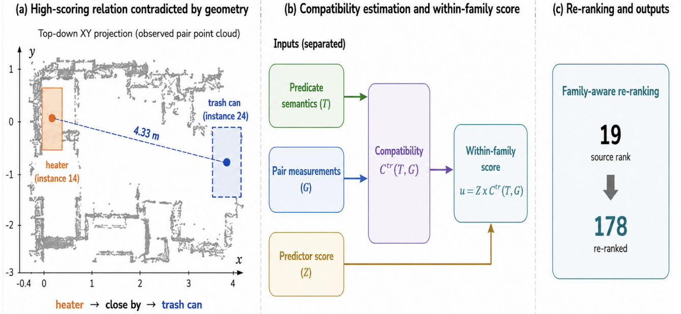
Figure 2: RelCompat3D overview. Predicate semantics T and predicate-independent geometric measurements of the ordered pair G determine C^{\text{tr}}(T, G) without the predictor score Z ; Z enters only in the within-family score u = Z \times C^{\text{tr}}(T, G) . Family-aware re-ranking moves the incompatible proximity example from rank 19 to 178.
