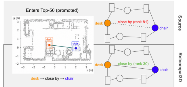
Figure 1: Open3DSG Top-50 promotion. An exact-label, verifier-satisfied desk close by chair candidate moves from rank 81 to 30; Table 1 reports aggregate results.
