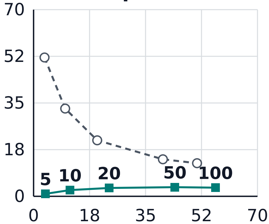
(b) Open3DSG
