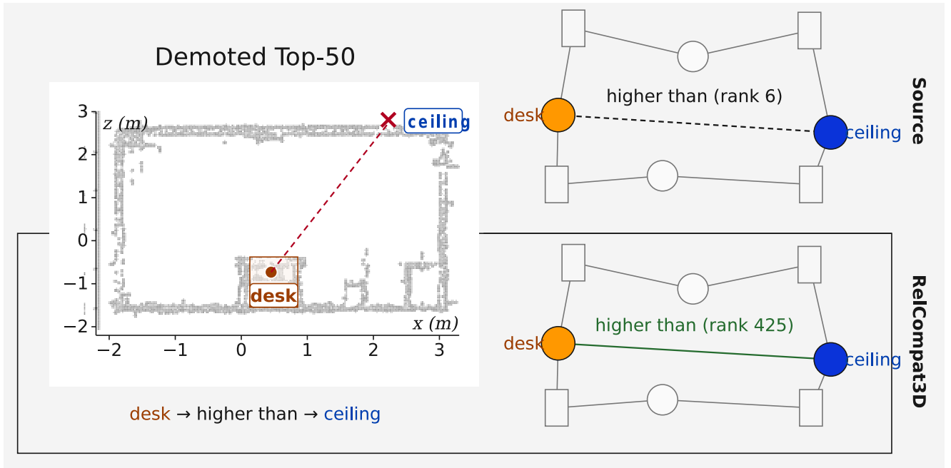
Figure 1: Open3DSG (Koch et al. 2024b) example. Measured elevation contradicts desk higher than ceiling ; family-aware re-ranking moves it from rank 6 to 425, outside the Top-50.
