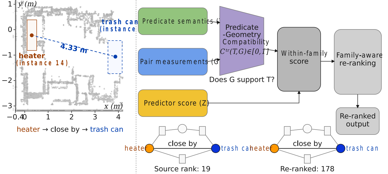
Figure 2: RelCompat3D overview. (a) Pair Geometry and Relation shows a high-scoring heater close by trash can prediction despite 4.33-m separation. (b) Compatibility and Re-Ranking computes C^{tr}(T, G) from predicate semantics T and pair measurements G without predictor score Z , then combines Z only in the within-family score, moving the relation from rank 19 to 178.
