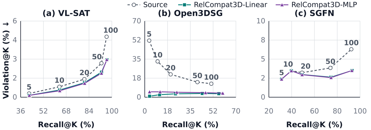
Figure 3: Recall@K–Violation@K trajectories. Each line connects K \in \{5, 10, 20, 50, 100\} for Source, RelCompat3D-Linear, and RelCompat3D-MLP. Rightward and downward movement is preferred. Numbers label K along the Source trajectory; all curves follow the same budget order. Axis ranges differ by predictor.
