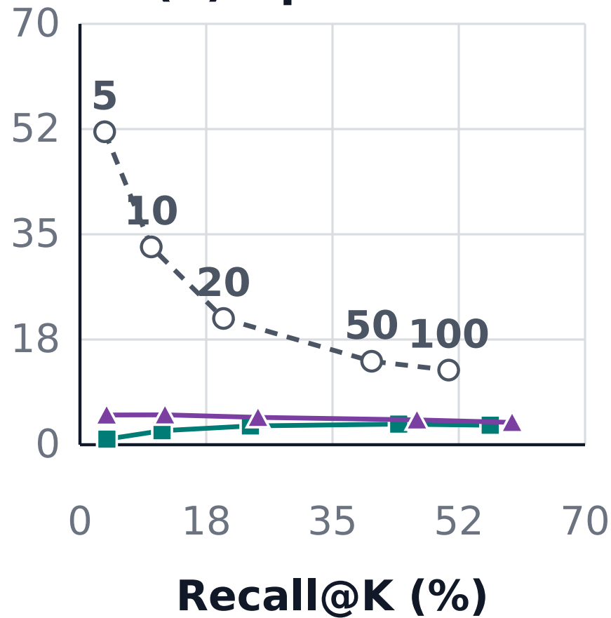
(b) Open3DSG
