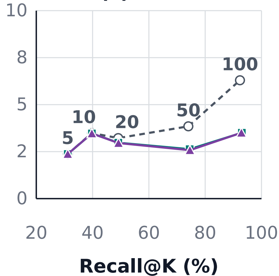
(c) SGFN
